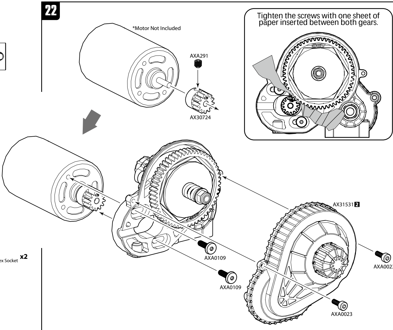
AXA0023 M2.6x8mm Cap Head x2
