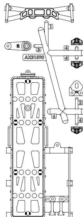
AX31590 Battery Tray and Servo Mount Set x1
